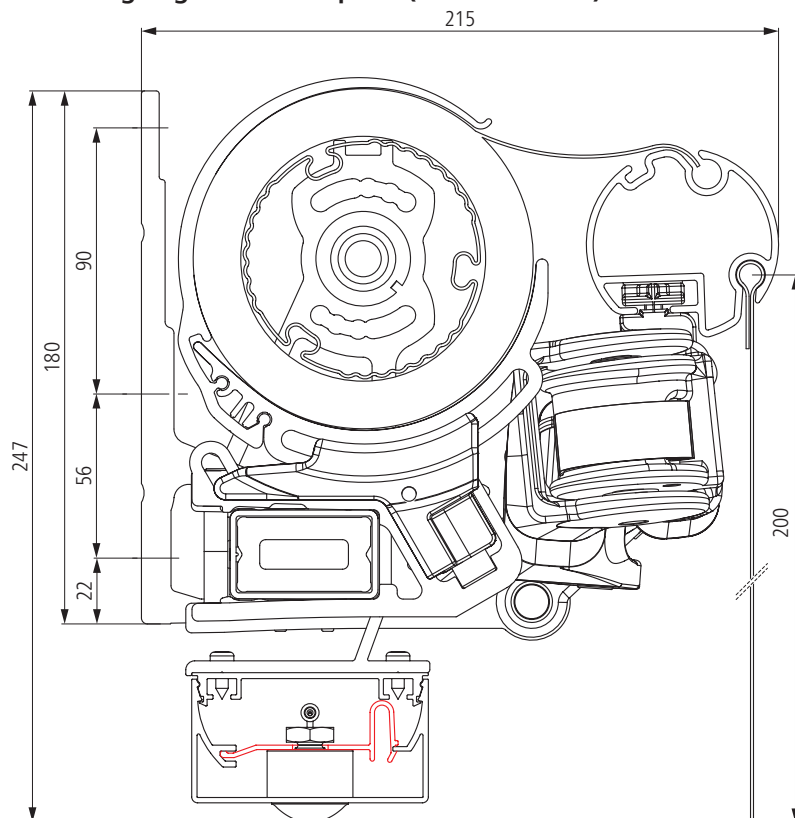
LED design light bar for Topas II (without a roof)
