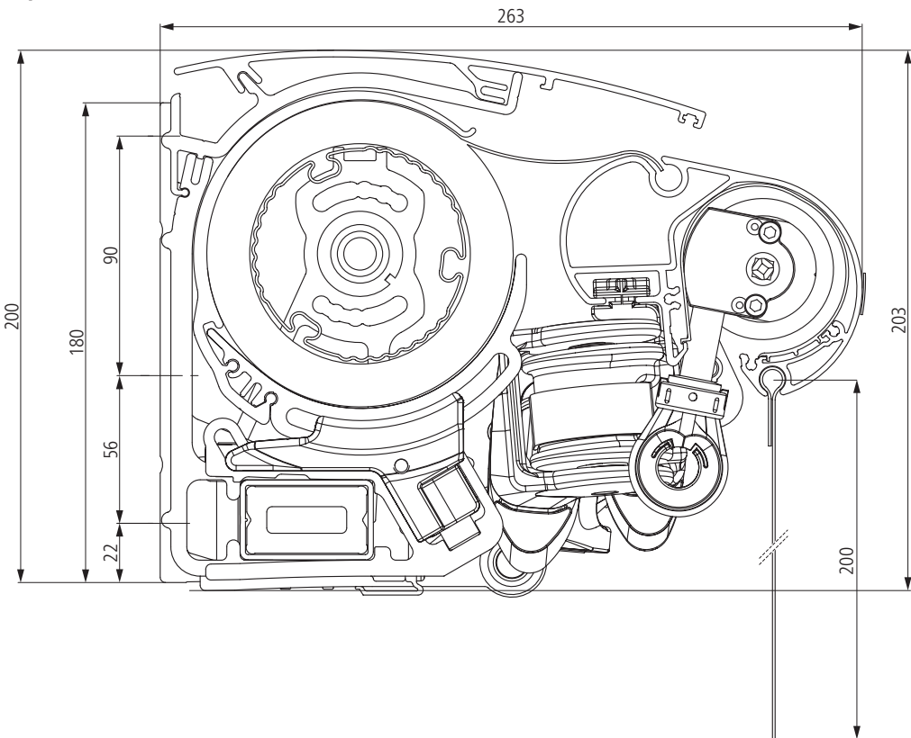
Topas II with a roof and VarioShade Valance crank drive
