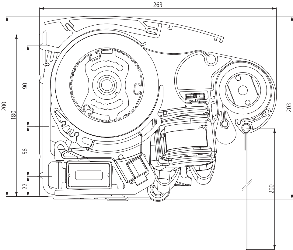
Topas II with a roof and VarioShade Valance motor
