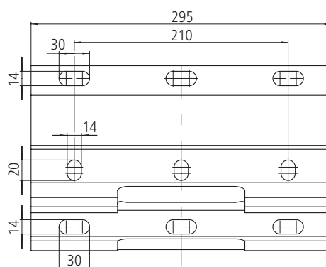
295 mm wall bracket (arm encapsulating)
