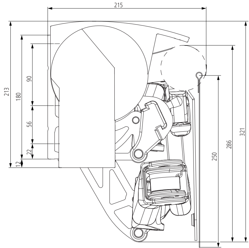
Topas II MiniMax with a roof
