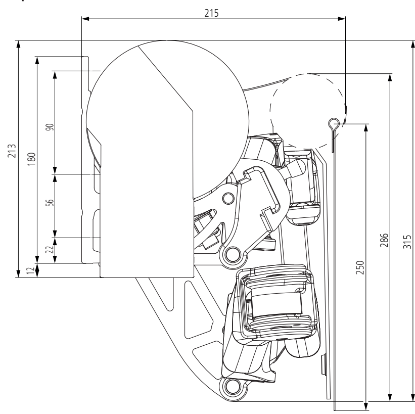
Topas II MiniMax without a roof
